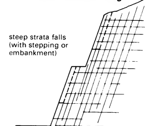
12 Geological influence on slope retention
